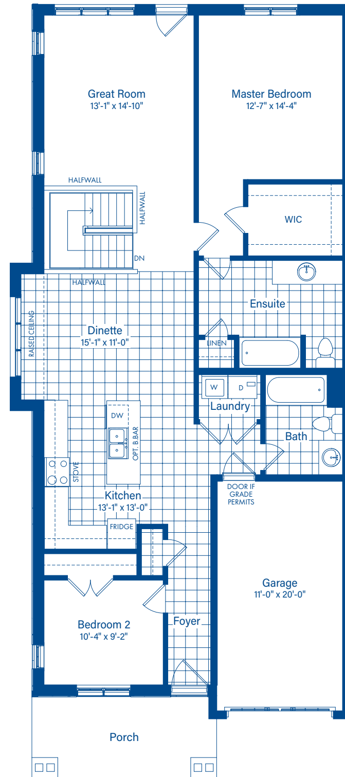
Main Floor Two Bedroom Plan
